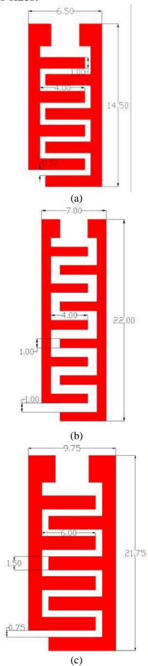
Fig. 1 - Design of Sensor (a), Sensor (b) and Sensor (c), respectively (all dimensions are in mm)
