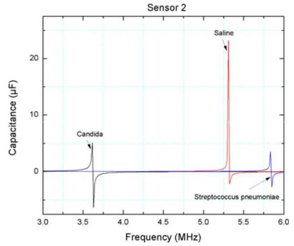
Fig. 5 Capacitance change of Sensor 2
