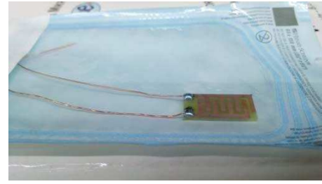
Fig. 2 Sensor after making contacts and after sterilizing
